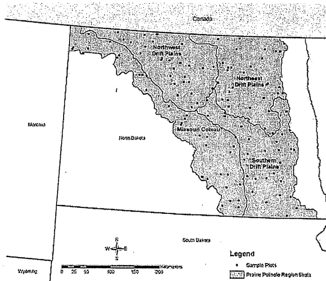
Figure 1. Sample sites in the stratified Prairie Pothole Region of North Dakota.
