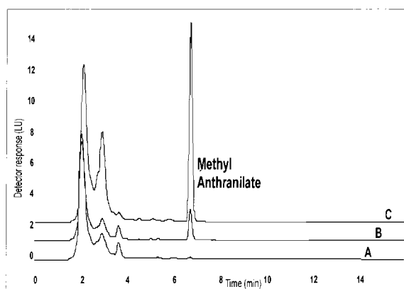
Figure 2. Comparative chromatograms of (A) control rice extract; (B) control rice fortified at 0.46 \mu\text{g/g} methyl anthranilate; and (C) a rice sample collected 5 days subsequent to the aerial application of Bird Shield bird repellent in Missouri rice fields (September–October 2002; the sample contained 2.80 \mu\text{g/g} methyl anthranilate).
