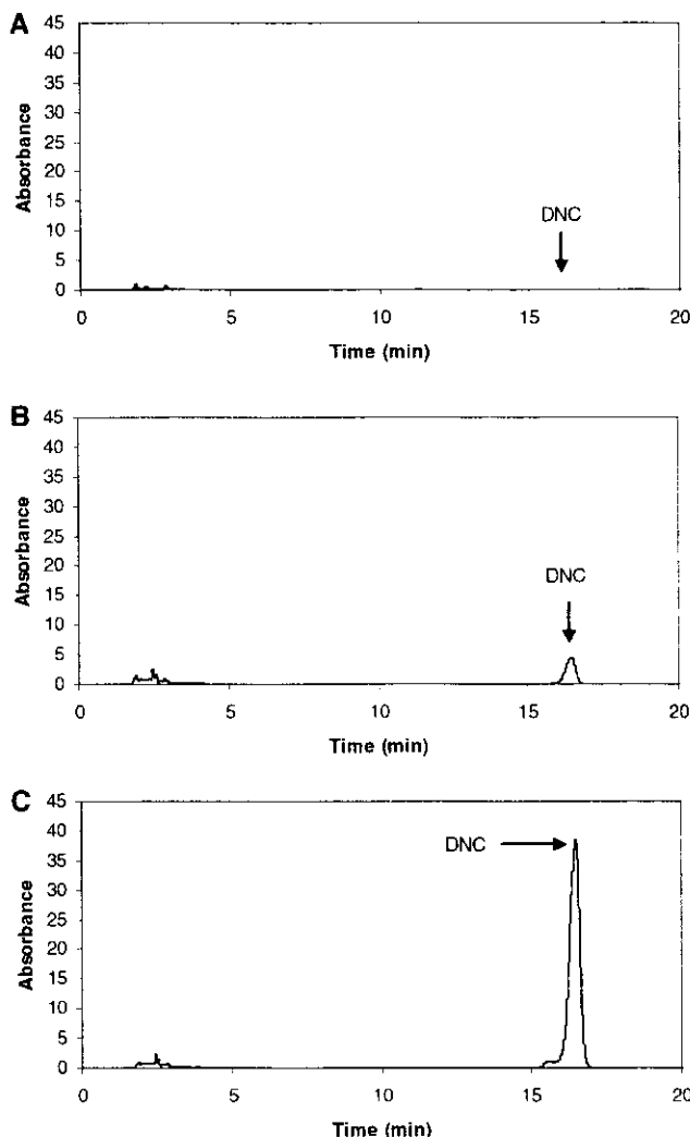
Figure 2. Chromatograms from DNC fortified chicken eggshell samples: control with no DNC (A); fortified at 0.0973\ \mu\text{g}/\text{g} (B); fortified at 0.986\ \mu\text{g}/\text{g} (C).
