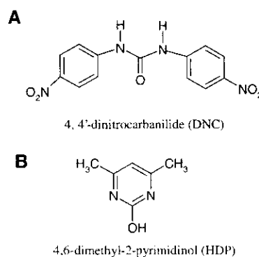
Figure 1. Structures of 4,4'-dinitrocarbanilide (DNC) and 4,6-dimethyl-2-pyrimidinol (HDP), the ingredients in Nicarbazin.
