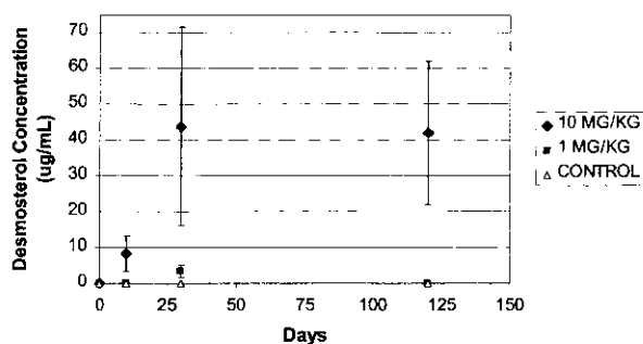
Figure 8. Mean ( \pm standard deviation) desmosterol concentrations in deer plasma.
