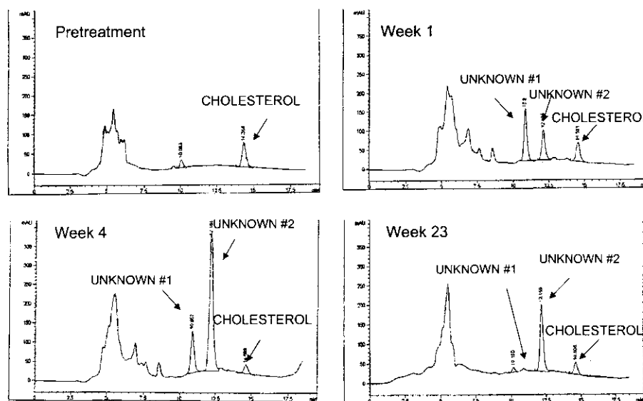
Figure 3. Sterol analysis of blood plasma from quail treated with 20,25-diazacholesterol (retention times: unknown no. 1, 10.8 min; desmosterol, 12.1 min; cholesterol, 14.5 min).
