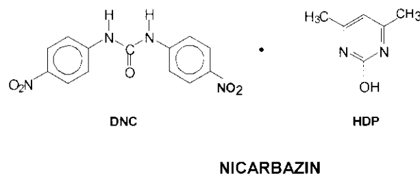
Figure 1. Nicarbazin.
