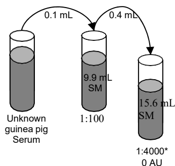
Figure 2. Dilution of the Unknown Guinea Pig Serum
