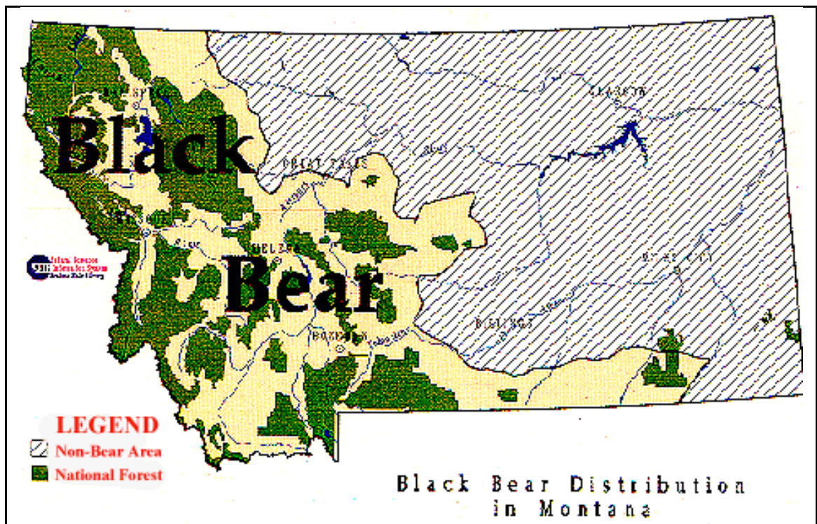
Figure 4-3. (Source: MFWP Final EIS Management of Black Bears in Montana)
