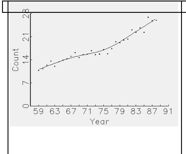
Figure 4-5. Raven Population Trend in Montana
