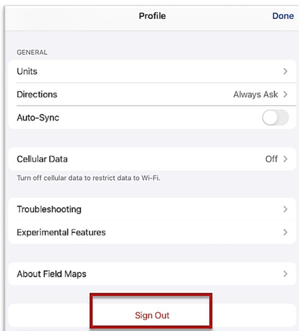
Figure 14. Profile Menu
