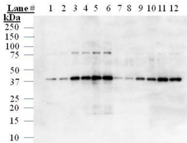
Figure C-3. Western Blot Analysis of MON 88701 DMO and E. coli -produced MON 88701 DMO Proteins
