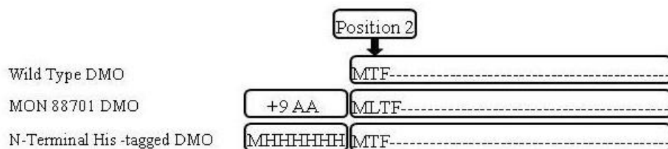
Figure C-1. Forms of DMO Protein and Their Relation to the Wild-Type DMO Protein
