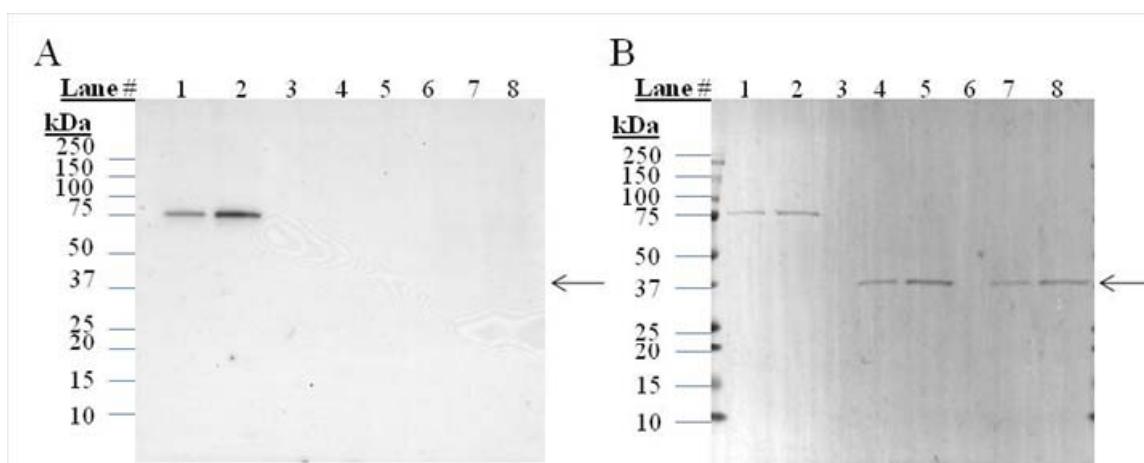
Figure C-5. Glycosylation Analysis of the MON 88701 DMO Protein
