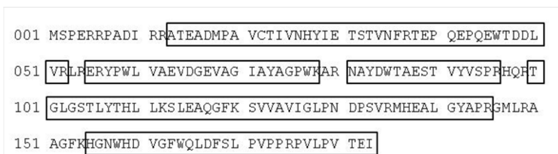
Figure C-10. MALDI-TOF MS Coverage Map of the MON 88701-produced PAT ( bar ) Protein
