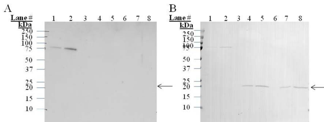
Figure C-13. Glycosylation Analysis of the MON 88701-produced PAT ( bar ) Protein
