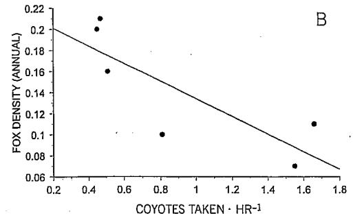
Fig. 3. Relationship between annual numbers of coyotes taken per hour in Utah versus kit fox density during the breeding season (A) and annual kit fox density (individuals \cdot km ^{-2} ) (B), U.S. Army Dugway Proving Ground, Utah.
