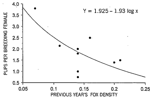
Fig. 1. Relationship between reproductive rate (pups per breeding female) of current year and annual fox density from previous year, U.S. Army Dugway Proving Ground, Utah.
